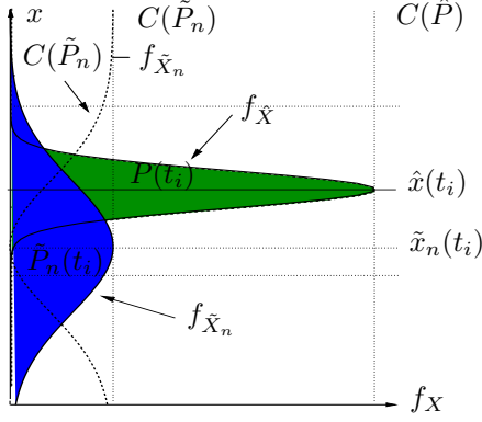
Fig. 1. A posteriori n -steps prediction likelihood (based on KL divergence).
