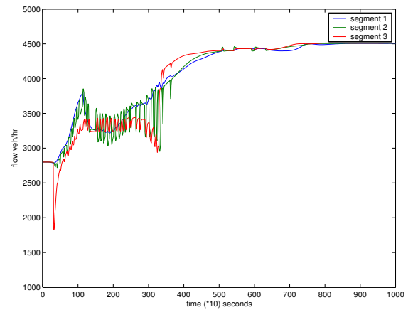
Fig. 5. Evolution of the flow on the segments of link L_{14} in the controlled case.
