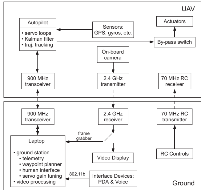
Fig. 7. System architecture
