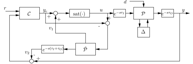
Figure 1: The proposed anti-windup scheme.
