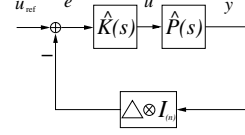
Fig. 2. The interconnected system with interconnection uncertainty.
