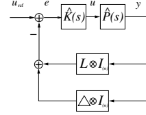
Fig. 3. The interconnected system with interconnection uncertainty.
