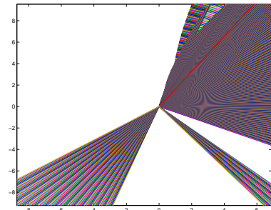
Fig. 6. The Nyquist-like plot of the interconnected system zoomed around -1+0j .
