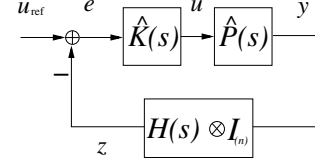
Fig. 1. The interconnected system.
