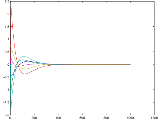
Fig. 7. Simulation results of the interconnected system with time-delays.
