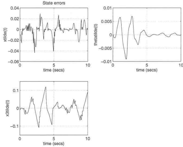
Fig. 4. Error in tracking (no disturbance).
