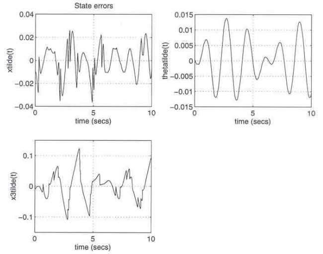
Fig. 7. Error in tracking (with disturbance).
