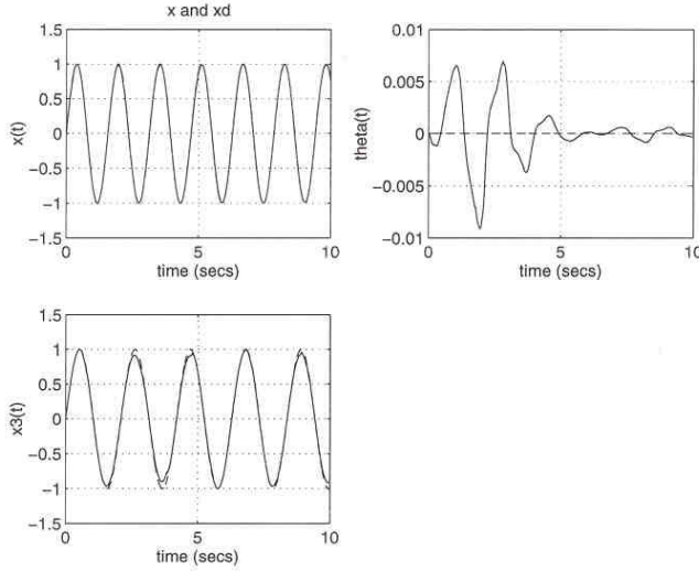
Fig. 3. Comparison of states (no disturbance).
