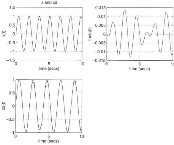
Fig. 6. Comparison of states (with disturbance).
