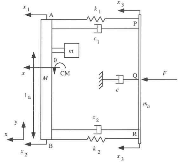
Fig. 2. Two-dimensional model of a CMM with the force F acting at Q .
