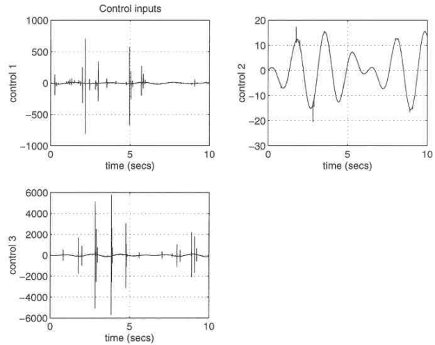
Fig. 5. Control inputs (no disturbance).
