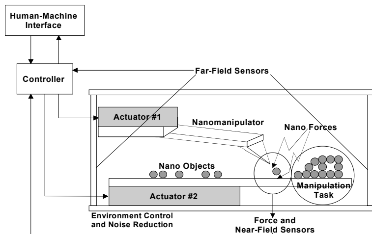
Figure 2 A generic robotic nano-manipulation system setup
