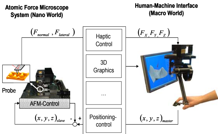
Figure 7 Direct teleoperation control based human-machine interface for an AFM
