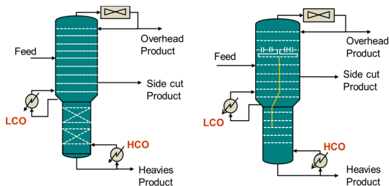
Figure 4a: Original Design of the FCC Unit Naphtha Splitter; Figure 4b: After Revamp to Proprietary DWC
