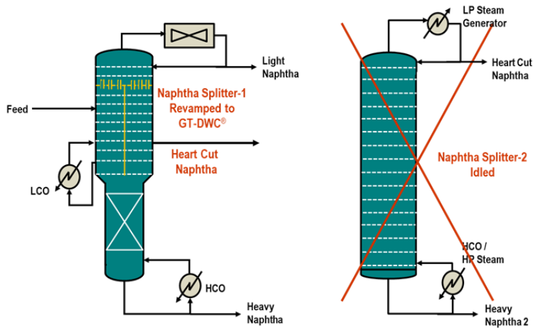
Figure 7: Naphtha Splitter-1 and Naphtha Splitter-2 after Revamp using Proprietary DWC
