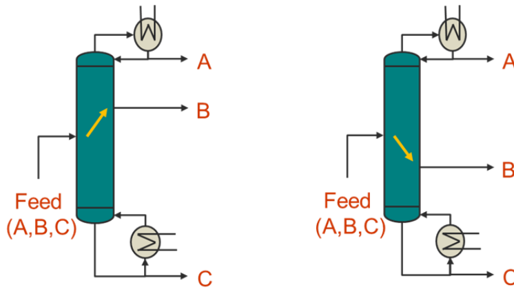
Figure 2a: Thermodynamic Inadequacies in Side-Cut Column for a Side-Cut above the feed; Figure 2b: Thermodynamic Inadequacies in Side-Cut Column for a Side-Cut below the feed.
