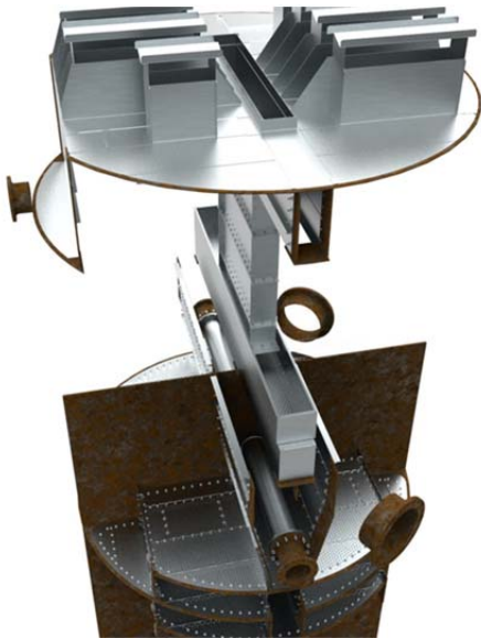
Figure 8a: Liquid Splitting Distributor in DWC column; Figure 8b: Dividing Wall Column Trays at Manufacturing Workshop
