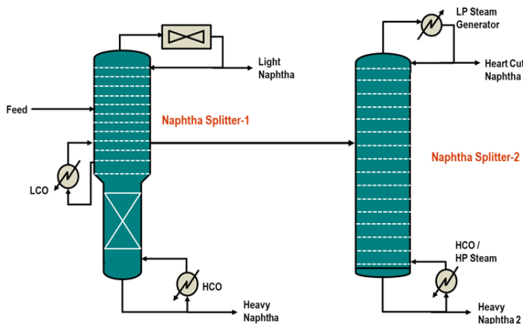
Figure 6: Original Design of Naphtha Splitter-1 and Naphtha Splitter-2
