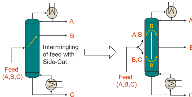
Figure 3: Conventional Side-Cut Column v/s Proprietary DWC
