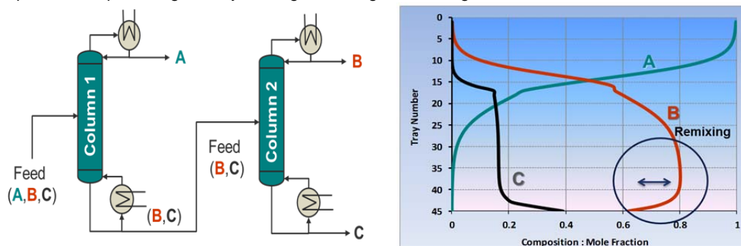
Figure 1a: Conventional Two-Column Separation; Figure 1b: Composition profile of components in a Two-Column Separation.
