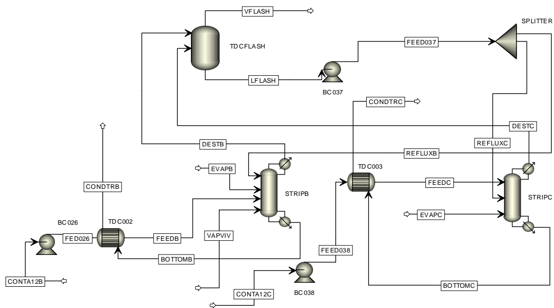
Figure 1: Example of a steam condensate treatment flowsheet designed by one of the students team.
