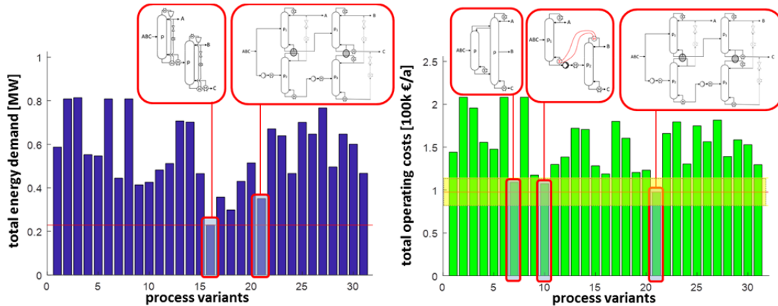
Figure 4: Illustration of the resulting total energy requirements (left) and total operating costs (right), for the separation of the ternary benzene, toluene, ethylbenzene mixture.
