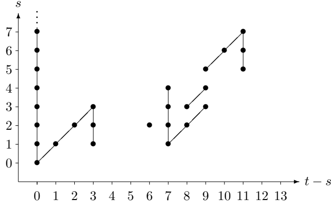
FIGURE 9. The ordinary Adams spectral sequence for [S^0, S^0]_* .
