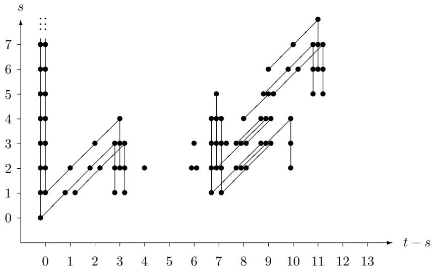
FIGURE 11. The Borel cohomology Adams spectral sequence for [S^0, S^0]^G
