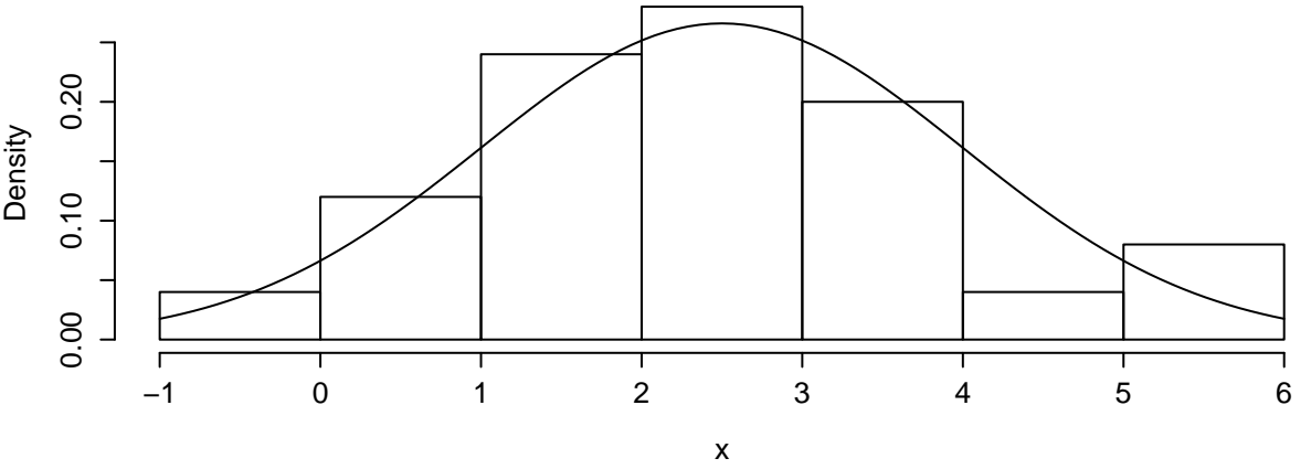
Histogram of x
