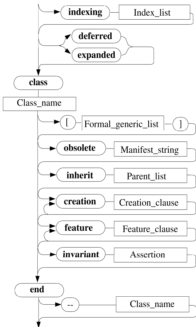
Class_declaration
