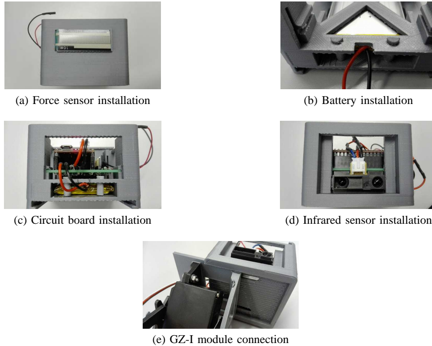
Fig. 4. Intermediate module assembly.
