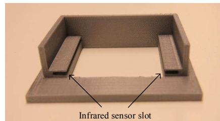
Fig. 5. Terminal module for head/tail infrared sensor mounting.
