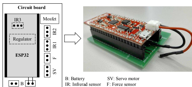
Fig. 8. Circuit board with an ESP32 Thing plugged in.
