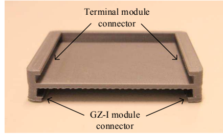
Fig. 6. Auxiliary module for connection between the GZ-I module and the terminal module.
