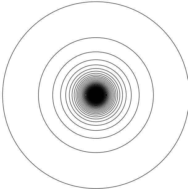
FIGURE 1. The set E , with n = 2 and \gamma = 0.7
