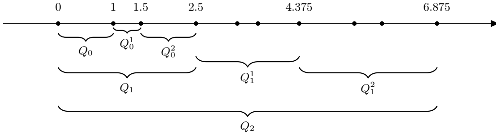
FIGURE 2. First steps of the construction of the set E
