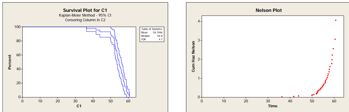
Figure 3: Kaplan Meier estimator and Nelson-plot from problem 3
