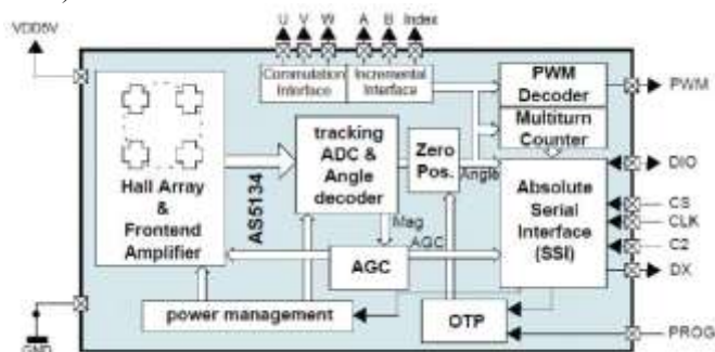
Fig.12. Block diagram of AS 5134 Hall Sensor (Austrian Micro Electronics 2010)
