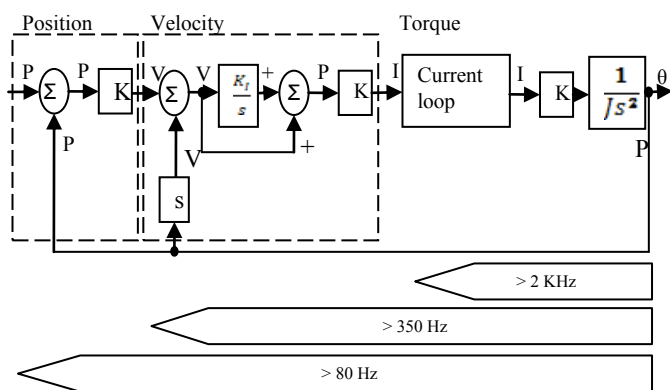
Fig. 5. Brushless motor's motion controller bandwidth (ELMO Company, 2010)
