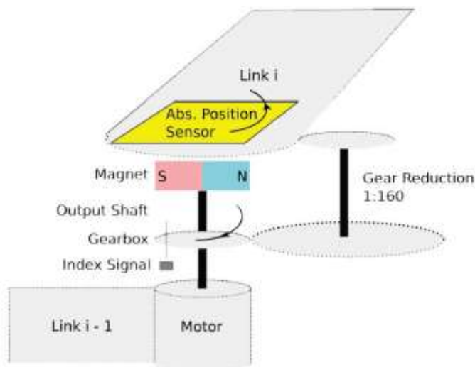
Fig.13. Contact less Absolute Positioning System
