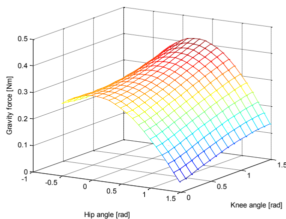
Fig. 7. Gravity force for swinging leg on knee and hip angle changing
