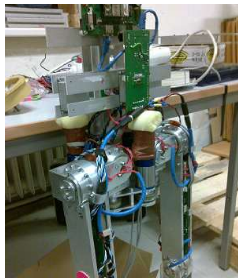
Fig. 4. Pelvis of the robot which contains eight motors (8 DOF)
