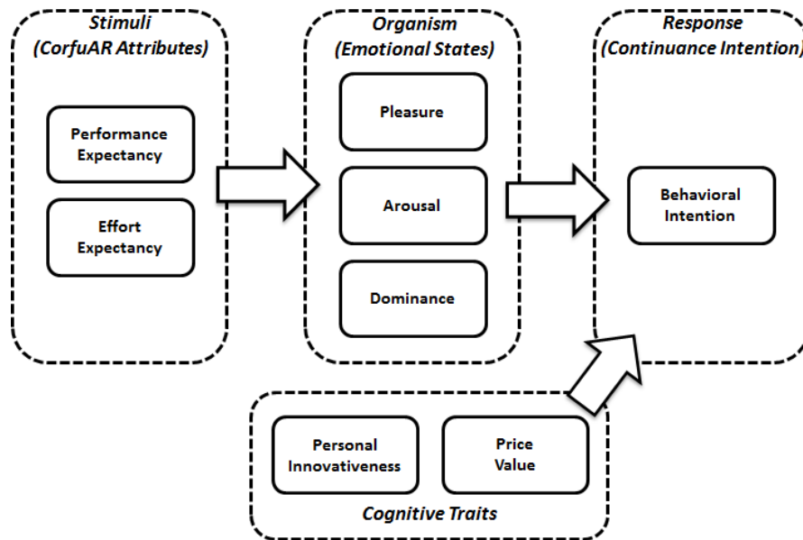
Fig 6 Research framework
