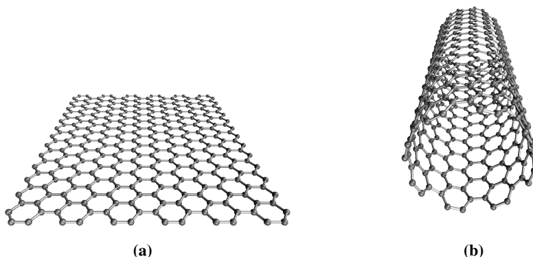
Figure 2.8: (a) A sheet of graphene consists of a single layer of carbon atoms arranged in a 2D honeycomb lattice. (b) A single-walled carbon nanotube (SWCNT) is obtained when a sheet of graphene is rolled up to form a cylinder. Figures derived from Eric Wieser, CC BY-SA 3.0, via Wikimedia Commons.
