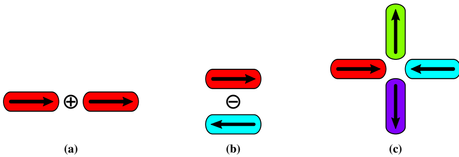
Figure 2.16: The relative arrangement of magnets determine the dipolar coupling between them. Shown here are two arrangements which results in a coupling where (a) aligned and (b) anti-aligned states are energetically favorable. (c) A geometrically frustrated system where all competing interactions cannot be satisfied at the same time. The state shown is one of the two configurations with the lowest energy. Colors indicate magnetization direction according to the color wheel in Fig. 2.14.
