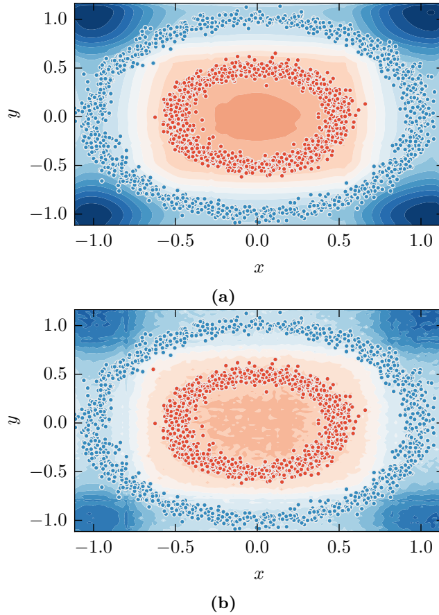
Figure 9: Decision surface and classification result on validation set: (a) simulation 100% accuracy (b) circuit 99.9% accuracy.
