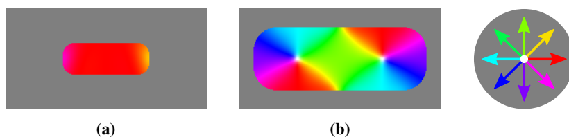
Figure 2.14: Internal magnetization of a (a) single-domain magnet and a (b) multi-domain magnet. The volume and shape of a nanomagnet determines its stable internal magnetization. Magnetization direction as indicated by the color wheel (white represents zero magnetization).
