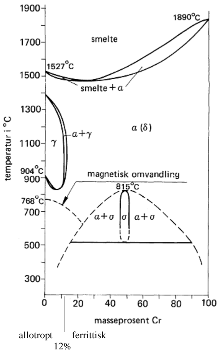
Figur 2.1 Fasediagrammet for jern-krom legeringer. (2)
